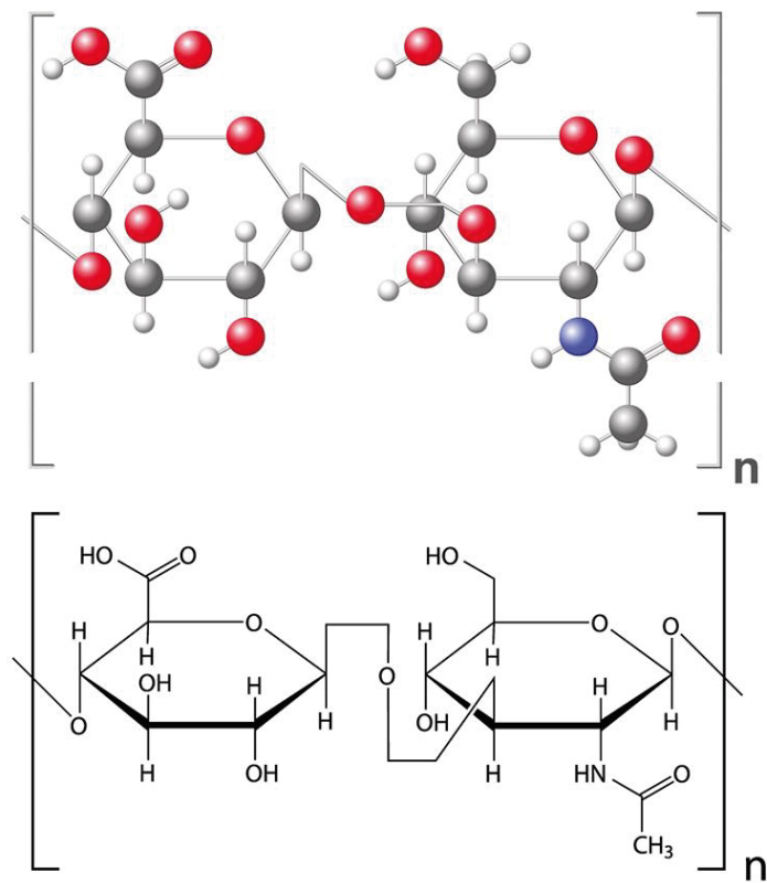
Chemical structure of Hyaluronic acid
